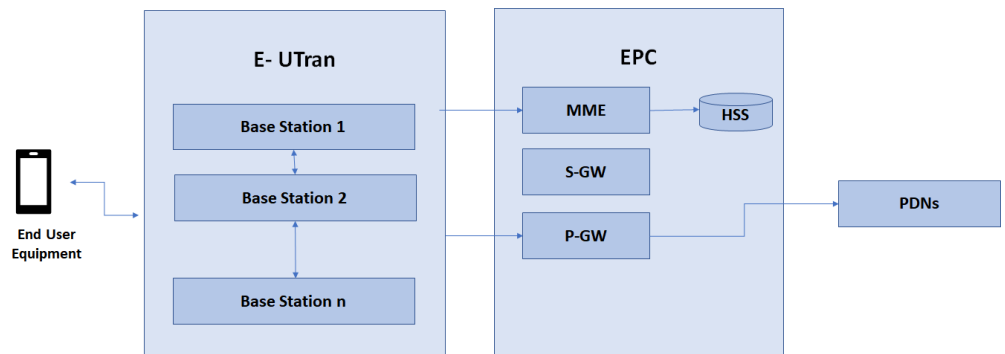
Figure 2 LTE Architecture
